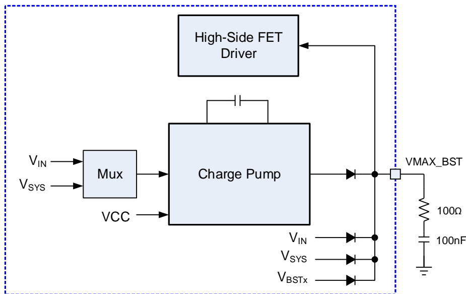
Figure 21: VMAX_BST Circuit Diagram
